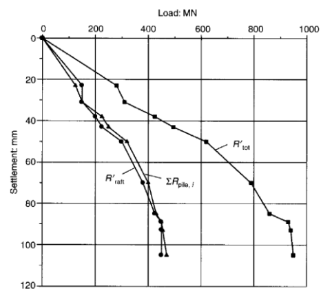
Figure 3.0 Observed load-settlement behaviour of raft, piles and total foundation system of Westend Tower Building (Katzenbach et al., 2000)
