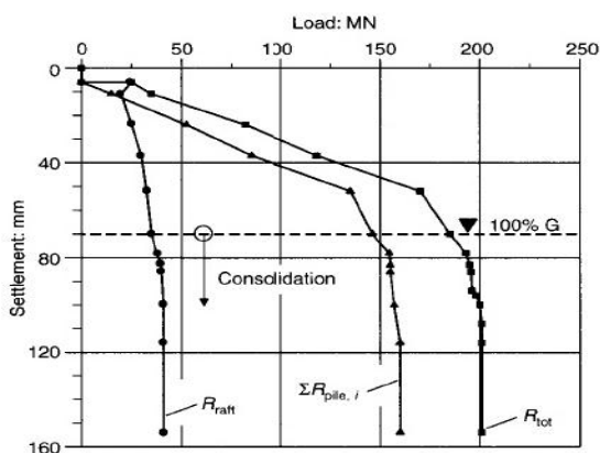
Fig. 1.0 Load Settlement curves
